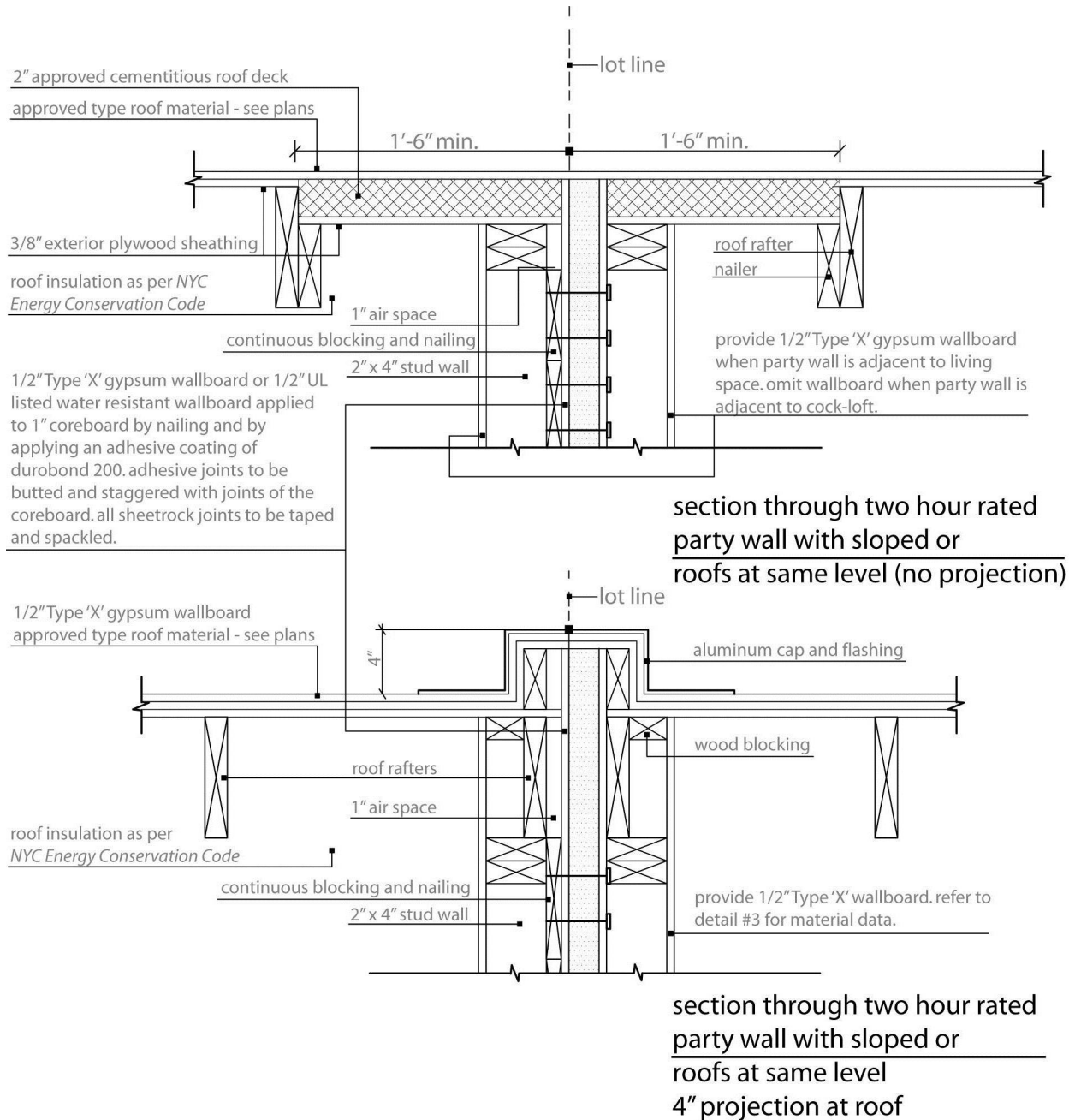
FIGURE M103(1) PARTY WALL VERTICAL SECTION
