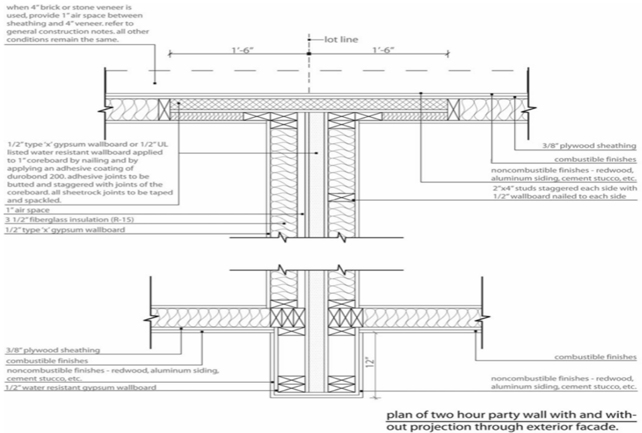
FIGURE M103(2) PARTY WALL PLAN SECTION
